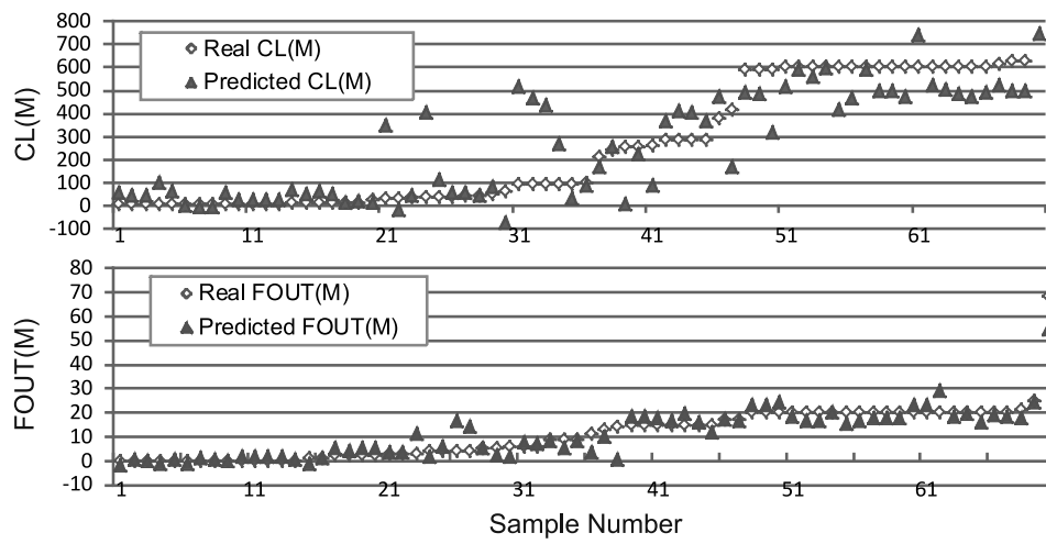
Figure 4: Comparison between the real and the predicted measures (according to the regression formulas) concerning the number of lines of code CL(M) and FOUT(M) ( n = 70 ).
