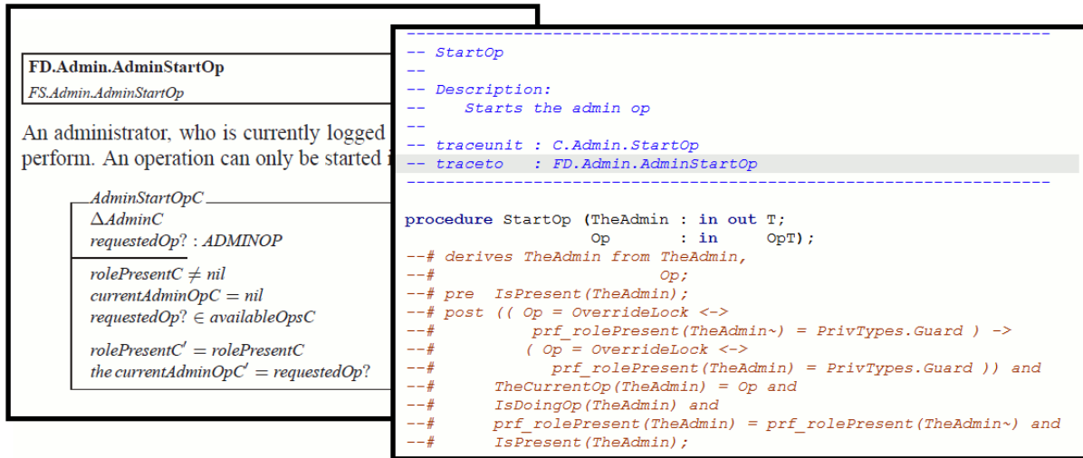
Figure 2: Snapshot of the Functional Design document (to the left) with unique identifiers for the units and the corresponding entry in the ADA specification file (to the right). This direct link enables the association between Z schemas and ADA modules.
