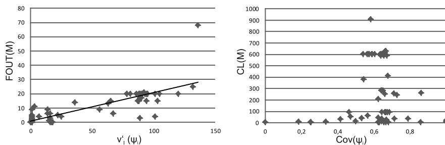
Figure 3: Scatter plots for the correlation between logical complexity v'_i(\psi) and FOUT(M) (left side) and for the correlation between coverage Cov(\psi) and Count Line CL(M) ( n = 70 ).
